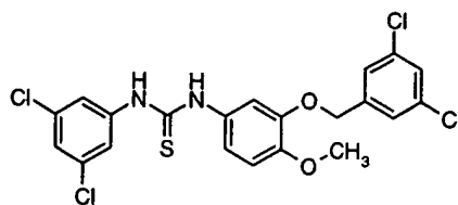
Compound # 28
